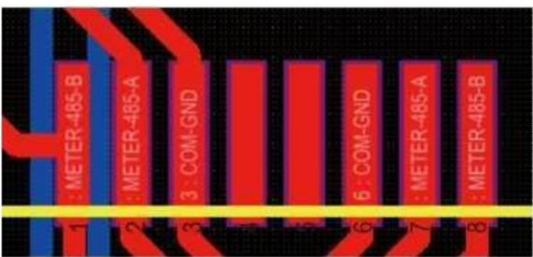
Meter-485-Port
